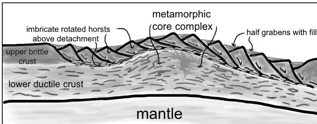
Figure 3.1-3: Generic Cross-section Showing Geologic Structure and Fault Geometries typical of the Basin and Range Province
